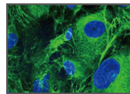
Collagen-I-alpha-1
